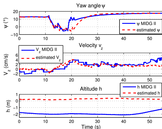
Fig. 12. Influence of magnetic disturbances with adapted gains (experiment)
