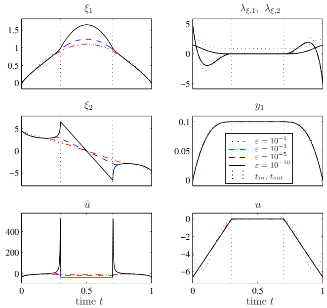
Fig. 4. Simulation results for \psi(\xi_1) \in \mathcal{C}^3 with decreasing \varepsilon and unboundedness of the junction points at t_{in}^- and t_{out}^+ for \varepsilon \rightarrow 0 .
